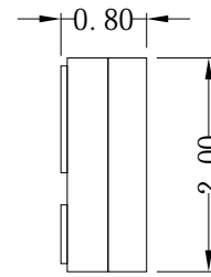
Fig.1-2 Side View
