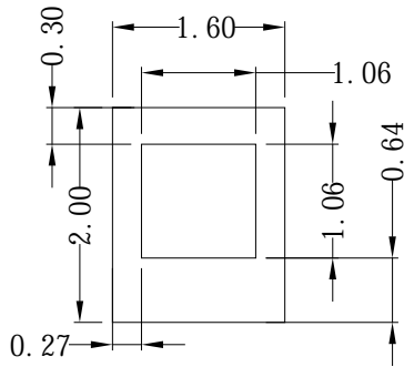
Fig.1-1 Top View
