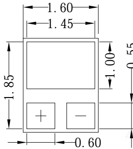
Fig.1-3 Bottom View
