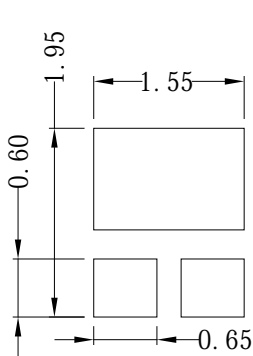
Fig.1-5 Soldering Patterns
